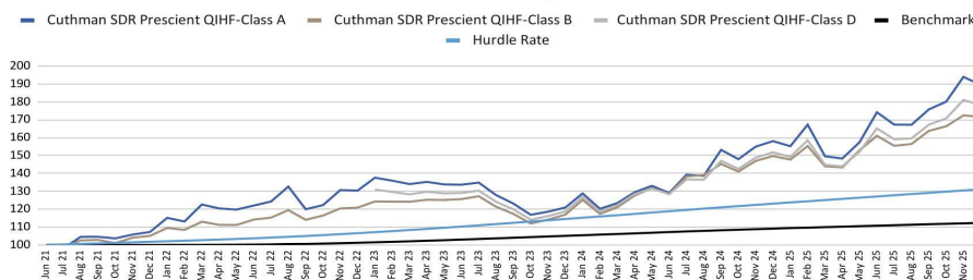
Total Return Since Inception - in SDR
