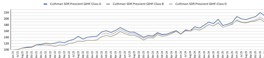
Total Return Since Inception - in ZAR
