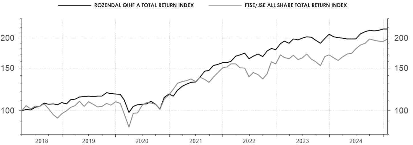
RELATIVE RETURN VS. BENCHMARK (REBASED TO 100) Source: Refinitiv Datastream
